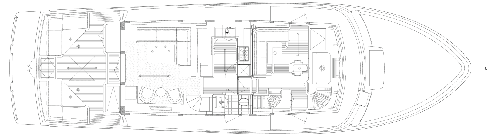
Main Deck
